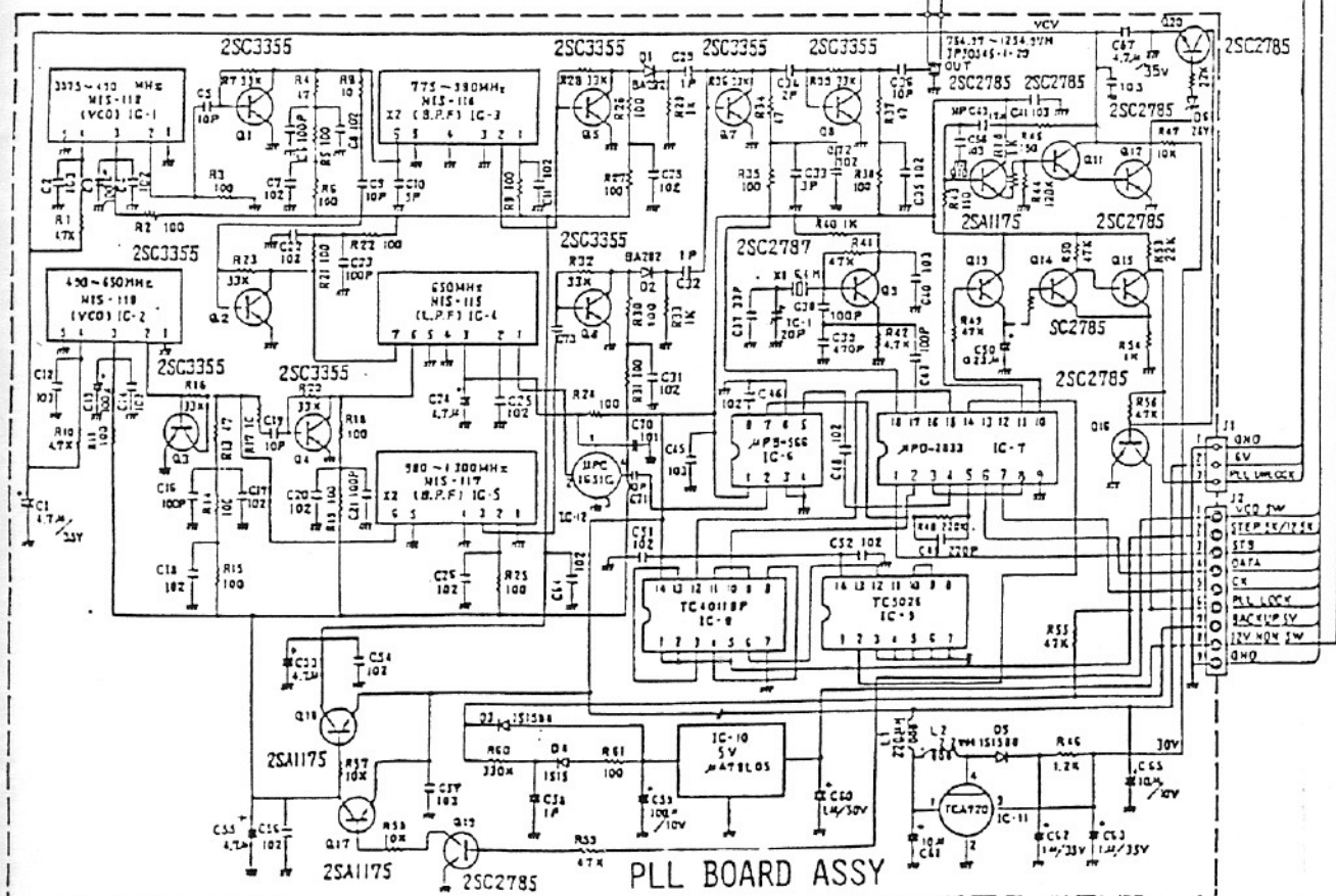
Figure 2.2 Schematic (Sheet 2 of 2) MY7000
